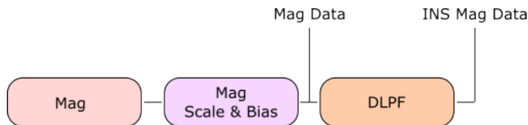
Figure 3: Magnetometer data flow.
